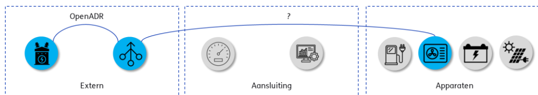
Figuur 4.11: Aggregator – apparaat variant
